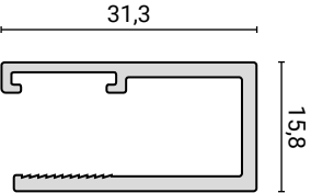
PROFILO A MURO WALL PROFILE WANDPROFIL PROFIL MURAL
